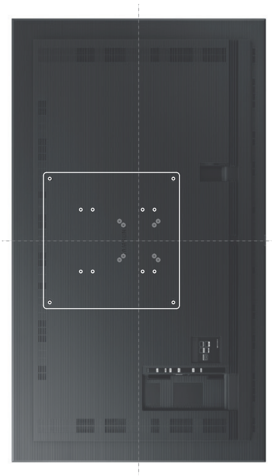
the decentralized arrangement of the VESA hole pattern is completely compensated by the adapter plate
